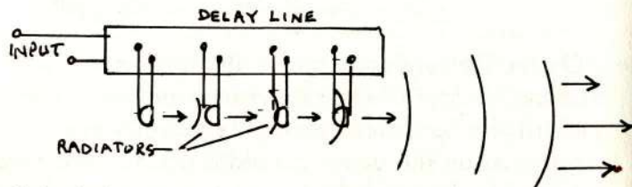
END-FIRE ARRAY ANALOGY WITH MODERN MICROWAVE GUIDE
