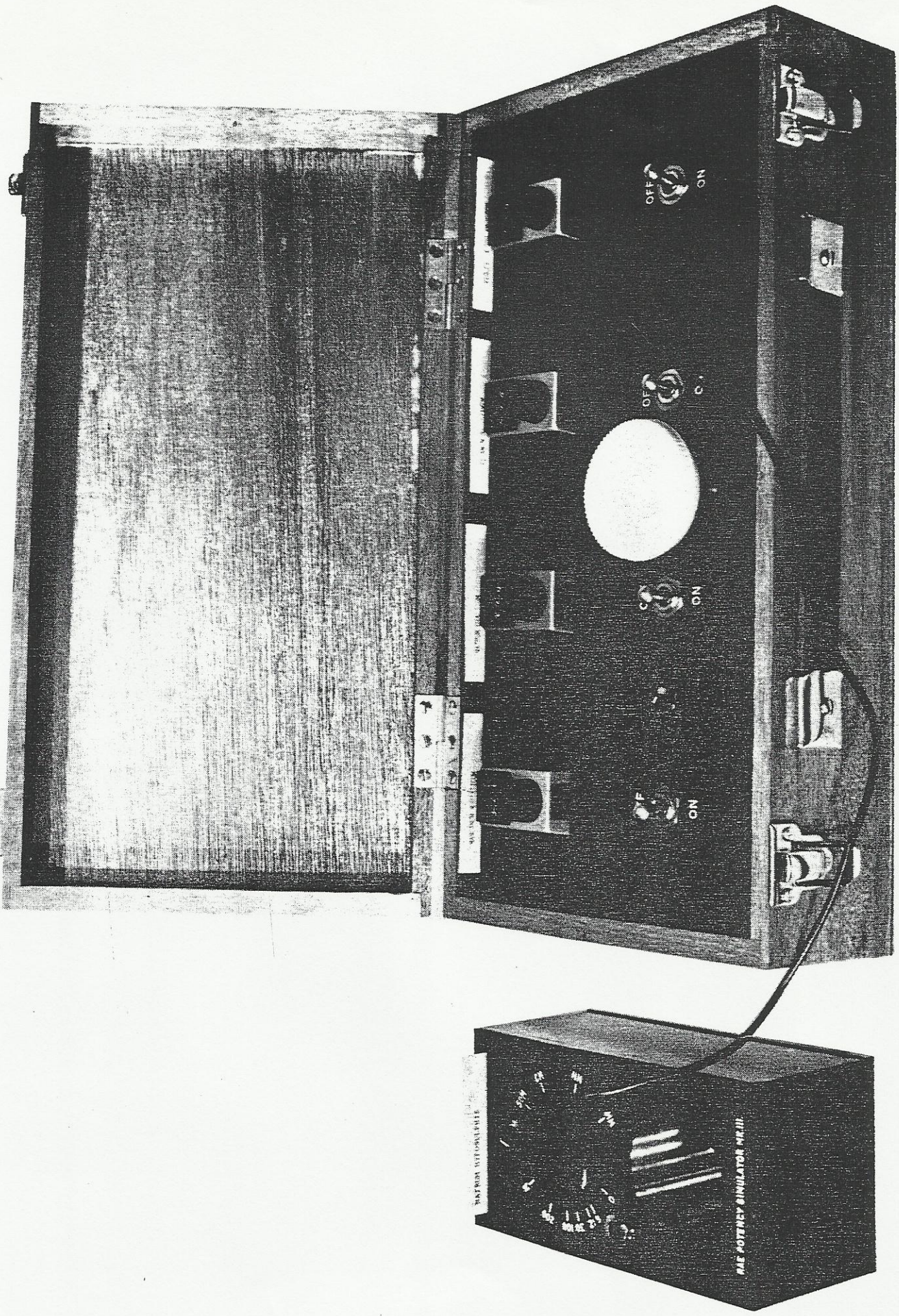
Fig. 24 A Potency Simulator connected to the Extended Range Multiple Potency Simulator
